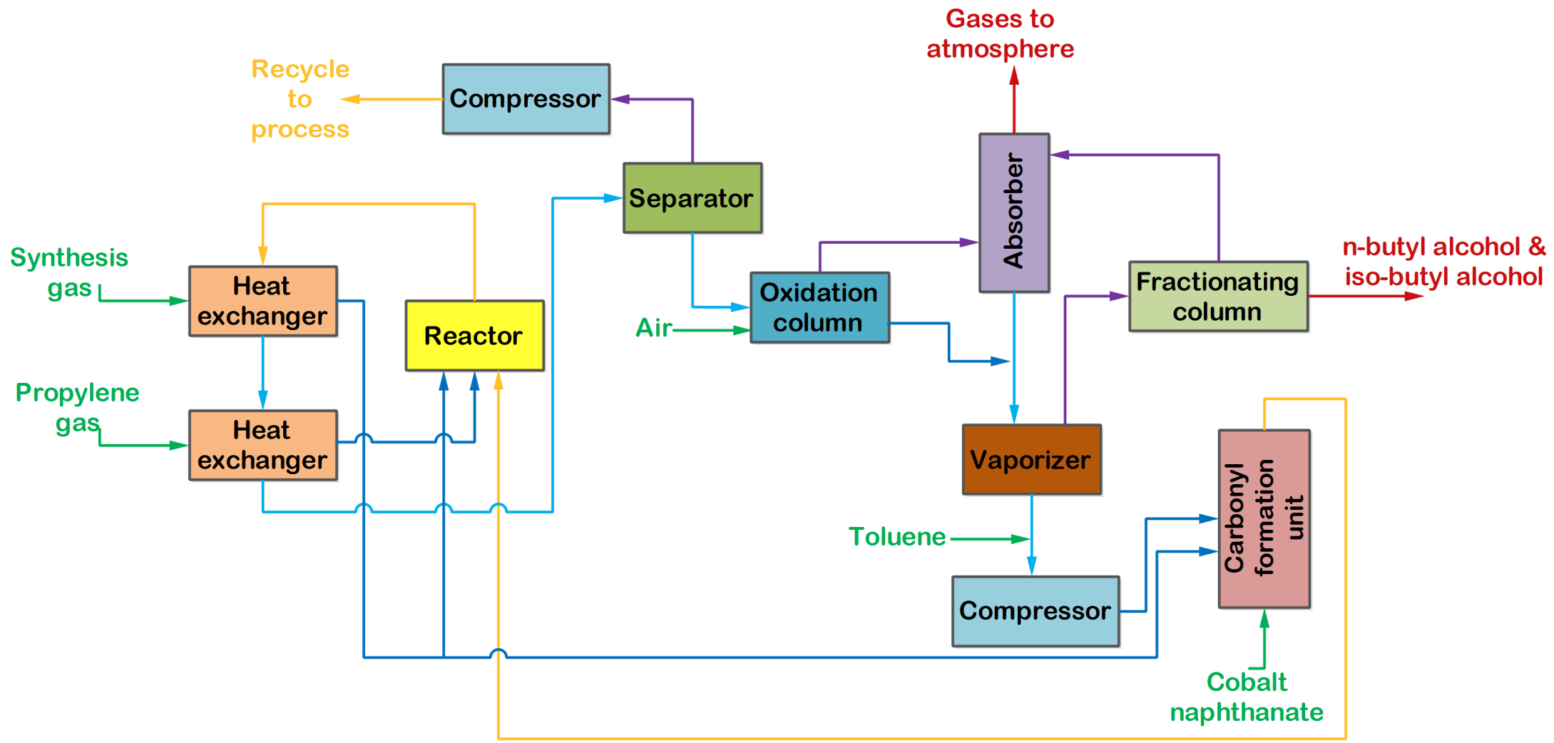
Figure: Manufacture of butyl alcohol from propylene and synthesis gas
